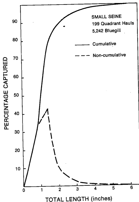
Figure 2. Relative length frequency of bluegill captured by seining in 27 CSPMWG ponds.
