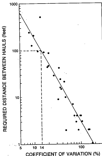
Figure 5. Effect of sampling variability, expressed as coefficient of variation of GM on the distance required between seine hauls to estimate the true shoreline abundance of small bluegill within \pm 10\% , assuming a 0.10 confidence level.
