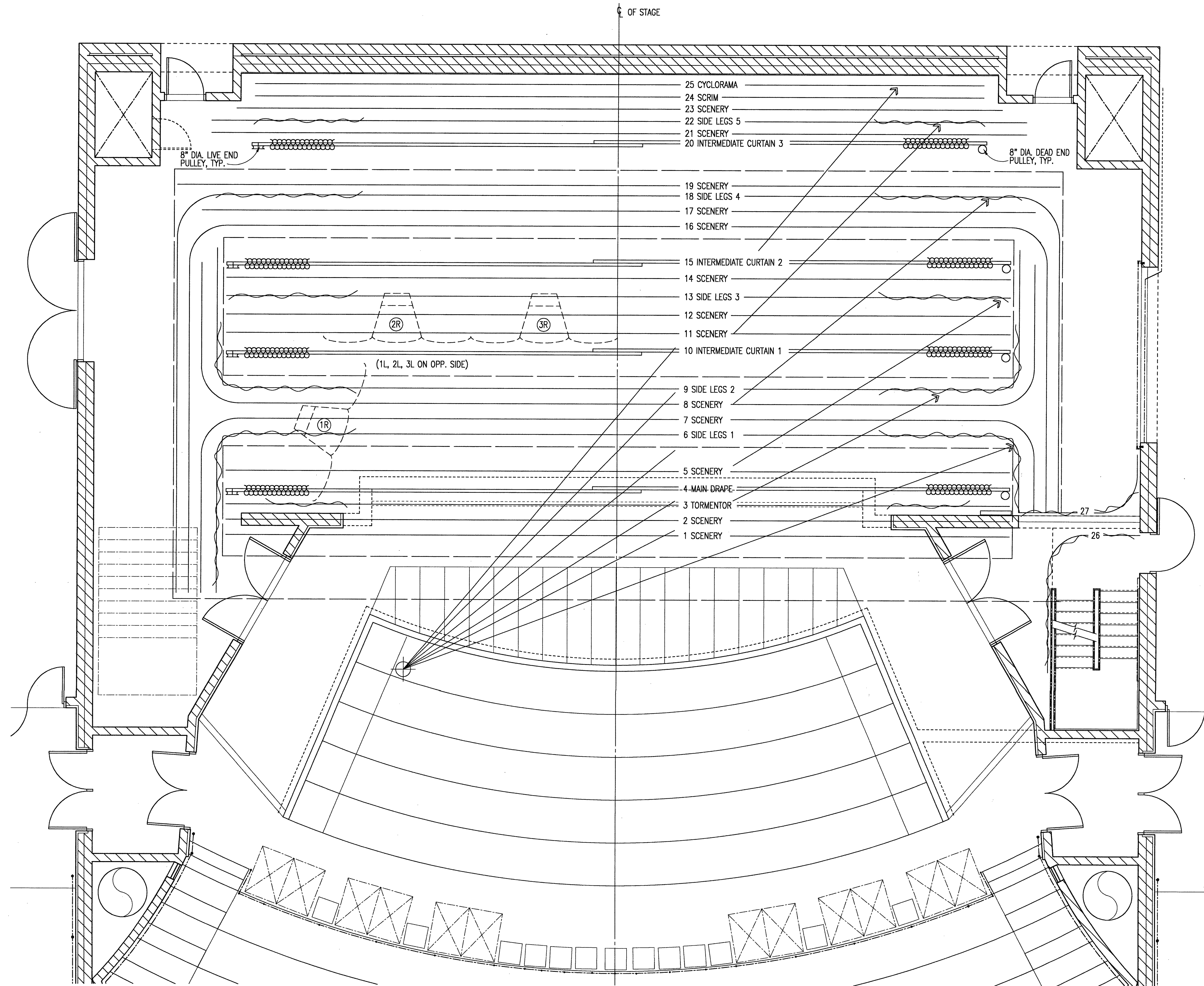
1. RIGGING PLAN SCALE: 1/4" = 1'-0"
